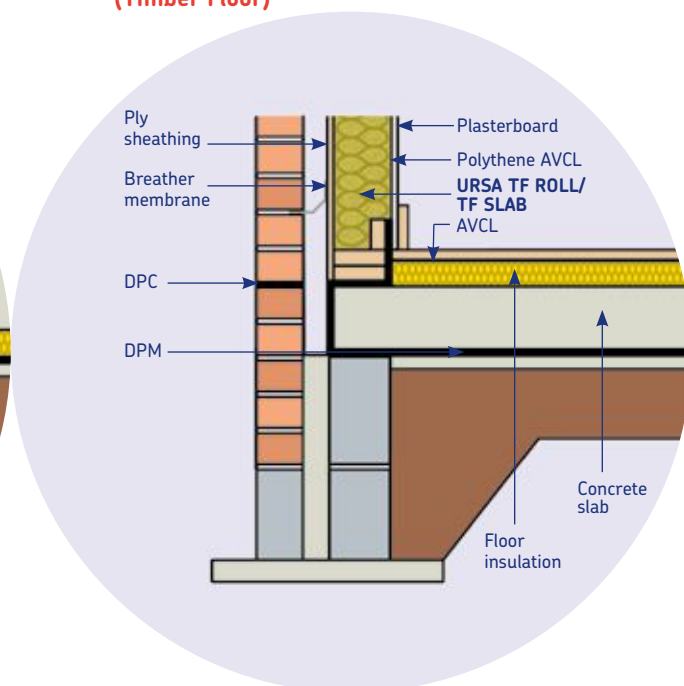
Figure 5 – Wall/Floor Junction Insulation Above Slab (Timber Floor)
