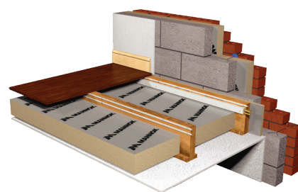
Suspended timber floor other than ground floor
