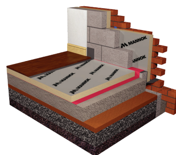
Solid ground floor: MF under timber floating floor
