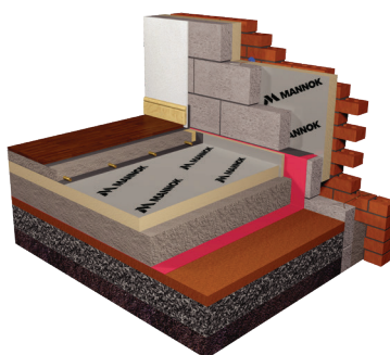
Solid ground floor: MF above groundbearing slab
