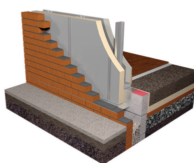
Cavity walls: MW in steel stud frame
